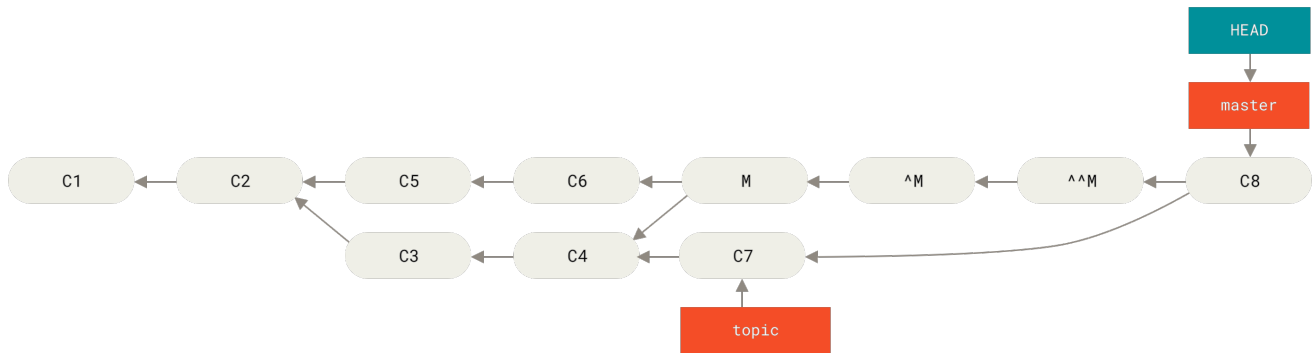
Figure 159. History after re-merging a reverted merge
