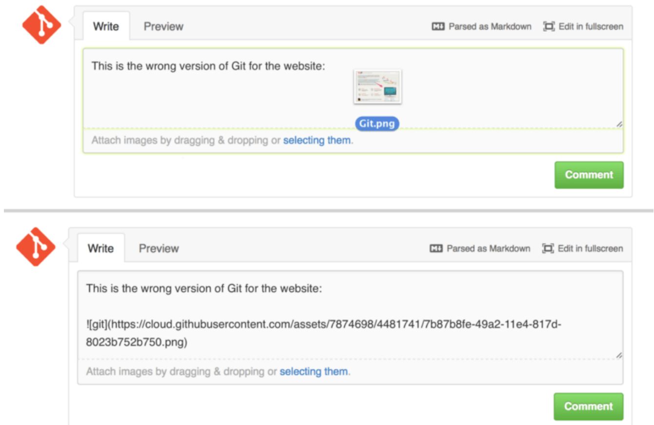
Figure 108. Drag and drop images to upload them and auto-embed them
