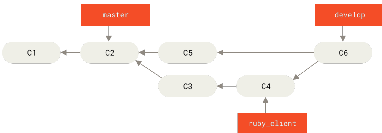
Figure 75. After a topic branch merge
