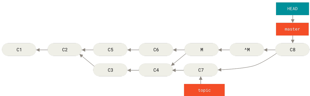
Figure 158. History with a bad merge
