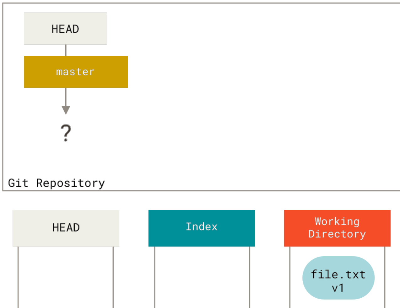
Figure 138. Newly-initialized Git repository with unstaged file in the working directory
