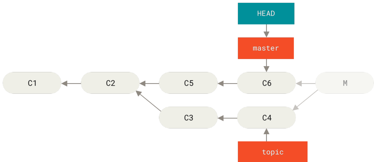
Figure 156. History after git reset --hard HEAD~
