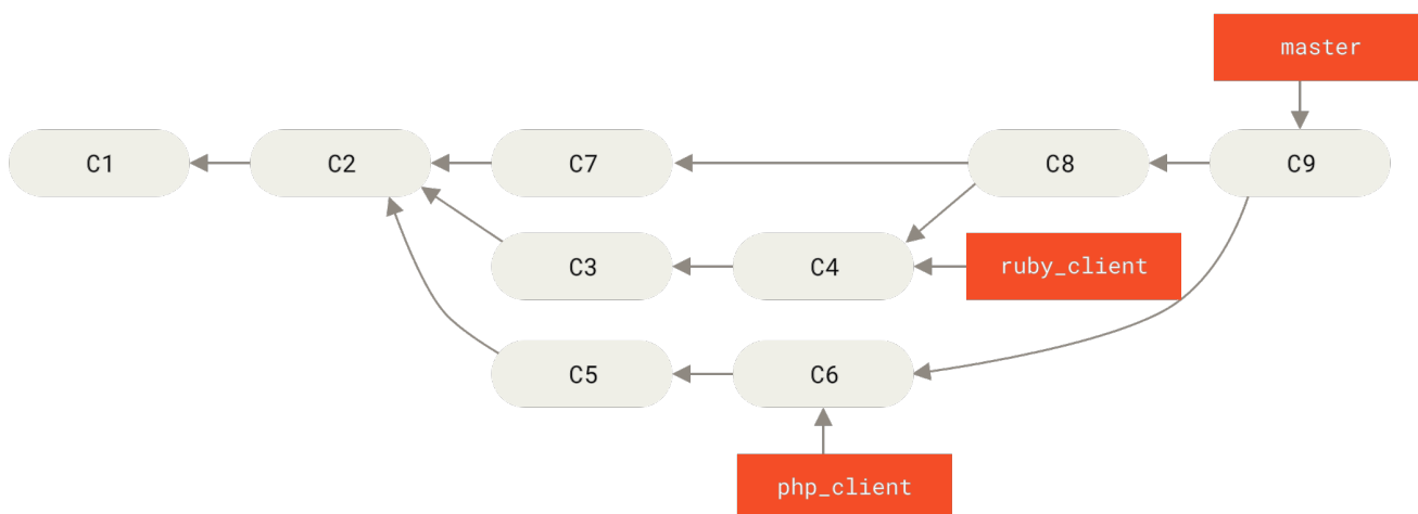
Figure 73. After a topic branch merge
