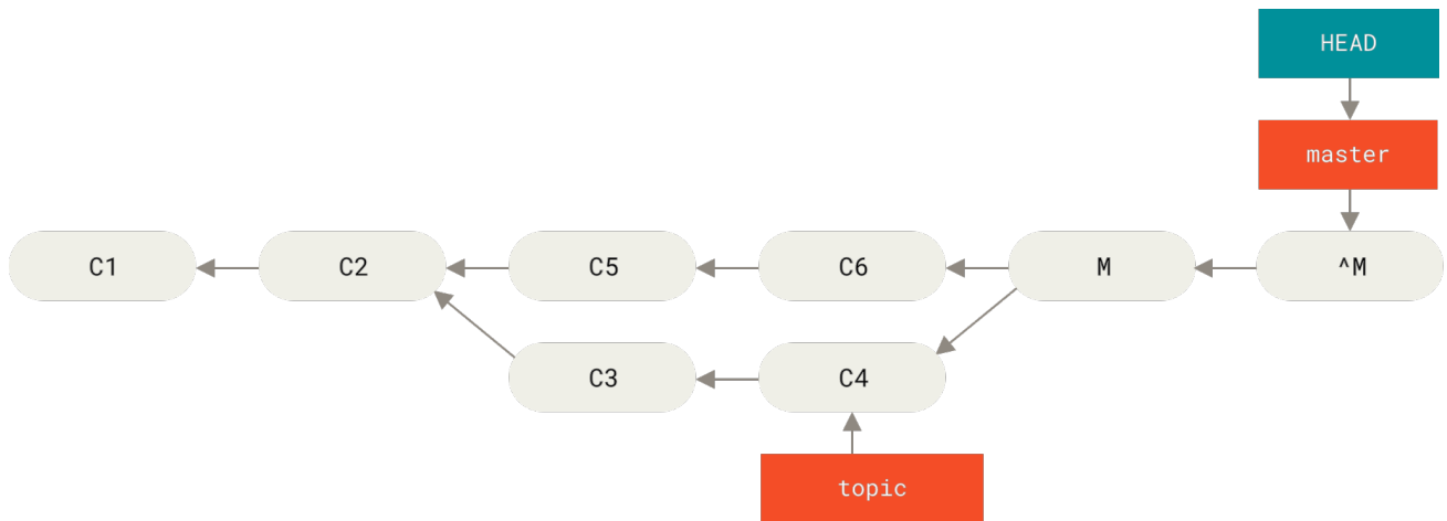
Figure 157. History after git revert -m 1
