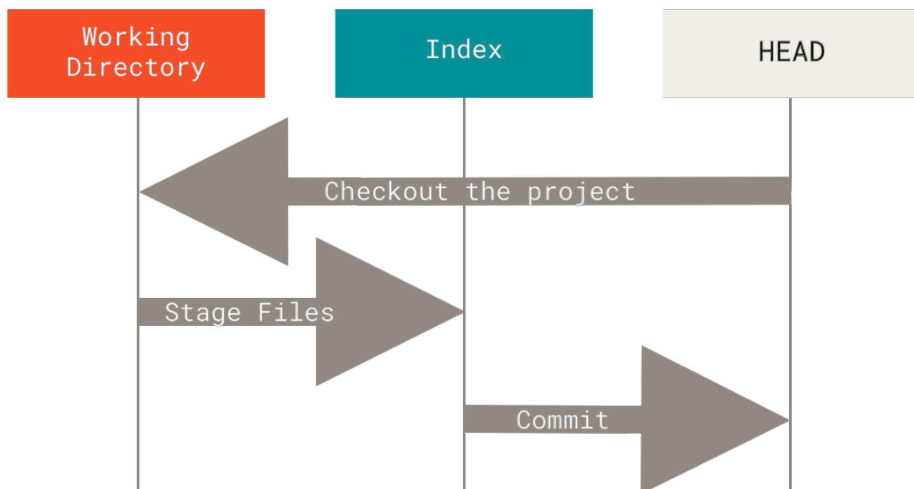
Figure 137. Git's typical workflow
