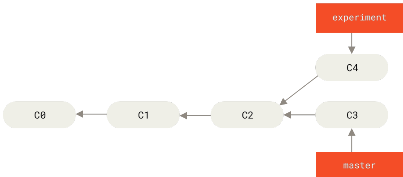
Figure 35. Simple divergent history
